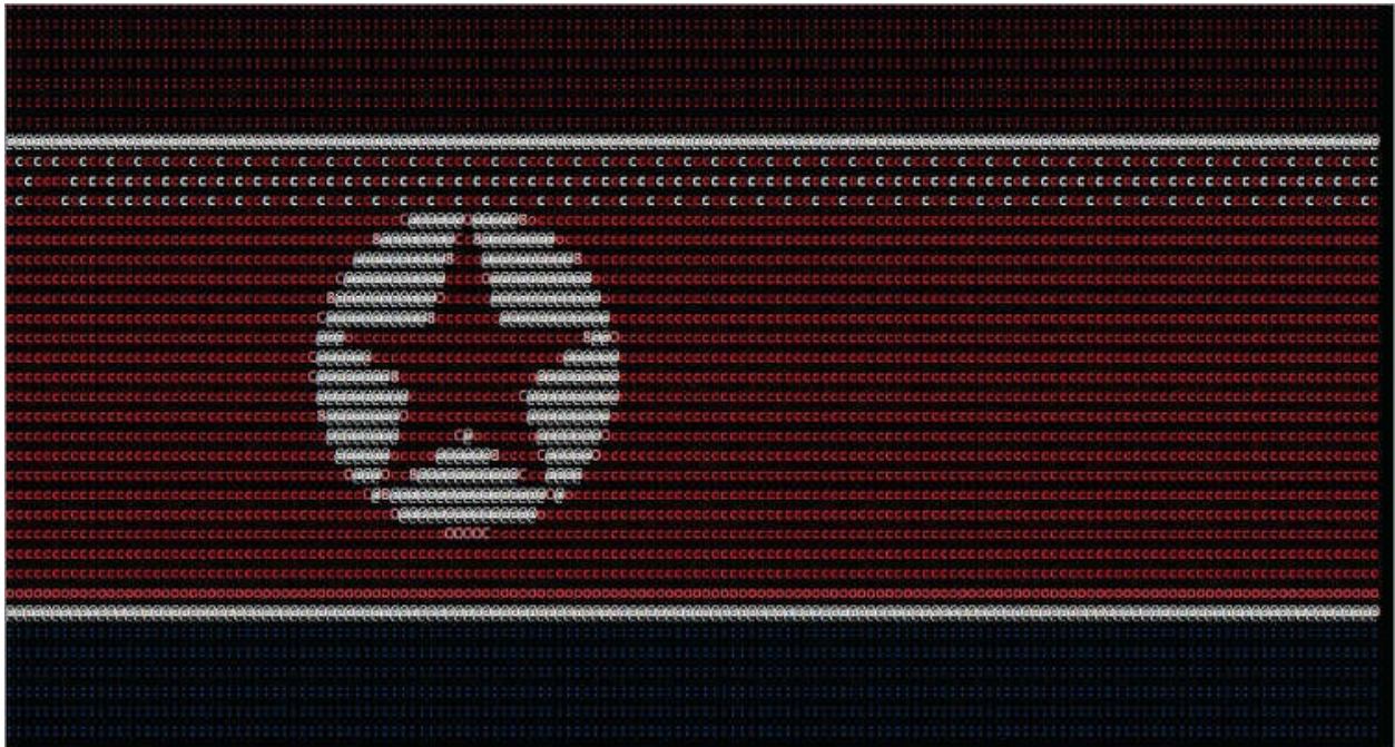
Figure 9.19: Old School!
