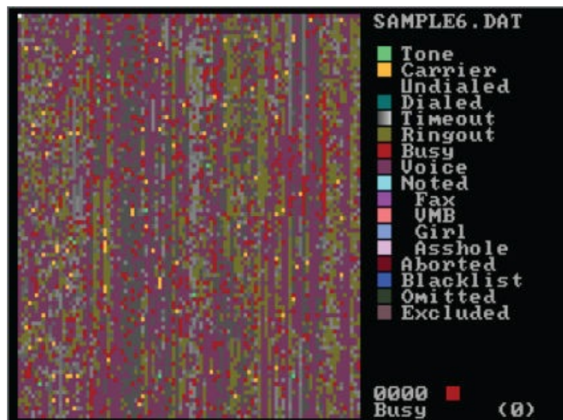
Figure 9.16: Toneloc output.
