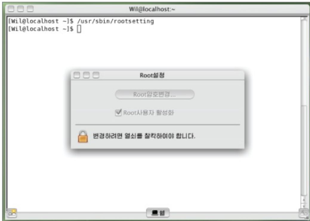
Figure 9.6: Run rootsetting.
