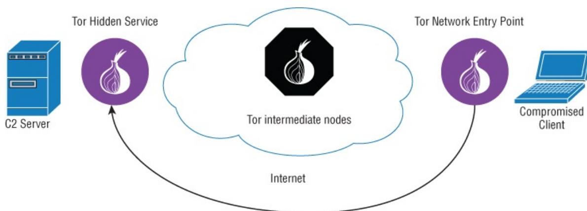
Figure 5.5: Simplified covert C2 topology.
