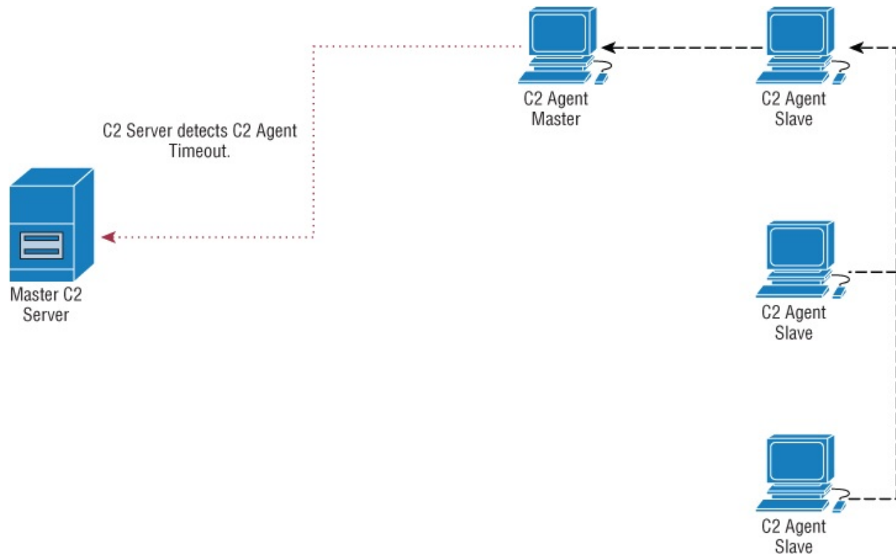
Figure 8.3: A timeout on the Master node signals it is likely no longer functional or the host is switched off.
