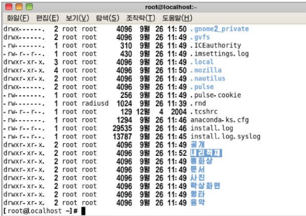
Figure 9.3: A shell.
