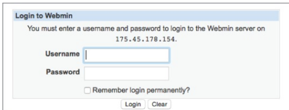
Figure 9.15: Webmin Interface.
