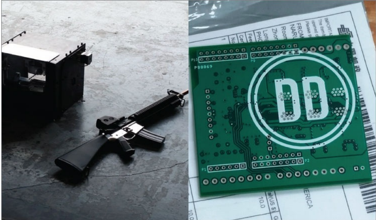
Figure 5.1: Defense distributed ghost gunner. An open source CNC machine designed to manufacture AR-15 lower receivers restricted under Federal law.
