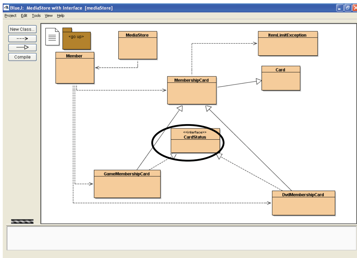
Figure 5.1 The class diagram for (a version of) the themed application
