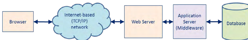
Figure 1-3 An n-tier web architecture
