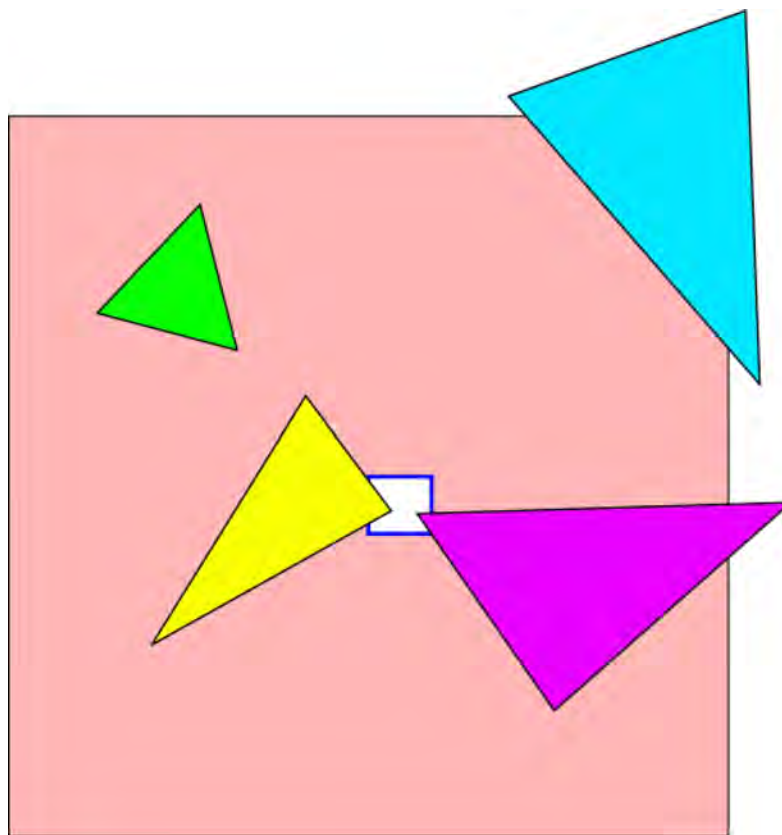
Guard-band clipping
