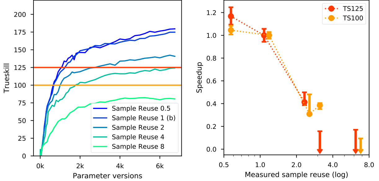
Figure 24: Effect of Sample Reuse on training speed. (Replicated from main text Figure 5c) TrueSkill over the course of training (see Appendix J) and speedup measured by the rate to attain different TrueSkill thresholds (computed using Equation 2) granted by increasing Sample Reuse. Increasing sample reuse causes significant slowdowns. In fact, the run with 1/8th as many rollout workers (sample reuse around 6.3), seems to have converged to less than 75 TrueSkill.
