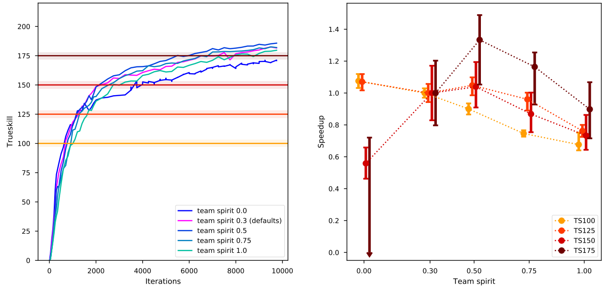
Figure 29: Team Spirit in early training: Very early in training (TrueSkill <125) the run with team spirit 0 does best; this can be seen by the speedup for lower TrueSkill being highest at team spirit 0. The maximum speedup quickly moves to 0.5 in the medium TrueSkill regime (150 and 175).
