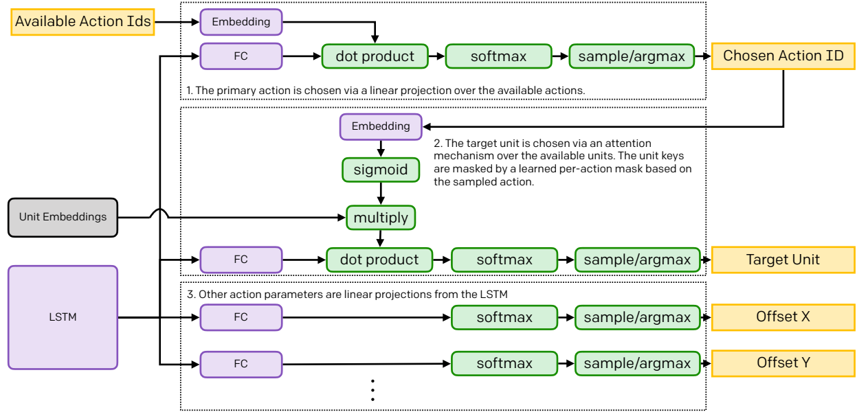
Figure 18: The hidden state of the LSTM and unit embeddings are used to parameterize the actions.
