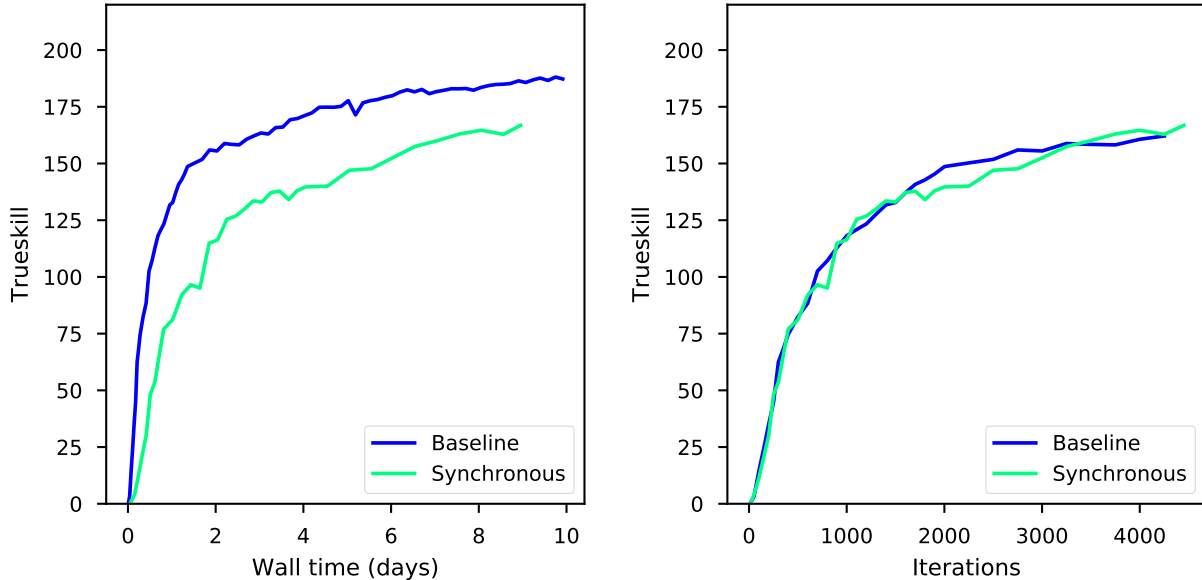
Figure 26: Asynchronous training: Plots of TrueSkill over the course of training for a “baseline” experiment together with a “synchronous” run using only on-policy data (staleness = 0) and restricting each sample to be used at most once (max sample reuse = 1). On the left, the x-axis is wall time. On the right, the x-axis is iterations. Asynchronous training is nearly 3x faster at achieving TrueSkill 150 when measuring by wall time, even though the two runs perform similarly as a function of the number of iterations.
