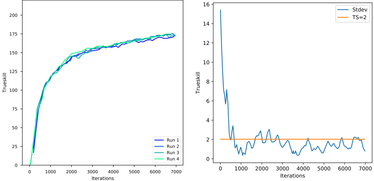
Figure 20: Variation in 5v5 baseline training: On the left, the TrueSkill over the course of training for different “baseline” experiments, using identical settings and hyperparameters. On the right, the standard deviation in TrueSkill across four runs. See Appendix C for the hyperparameters used. Although we only have 4 runs, we can estimate that different runs tend to vary by about 2 TrueSkill.
