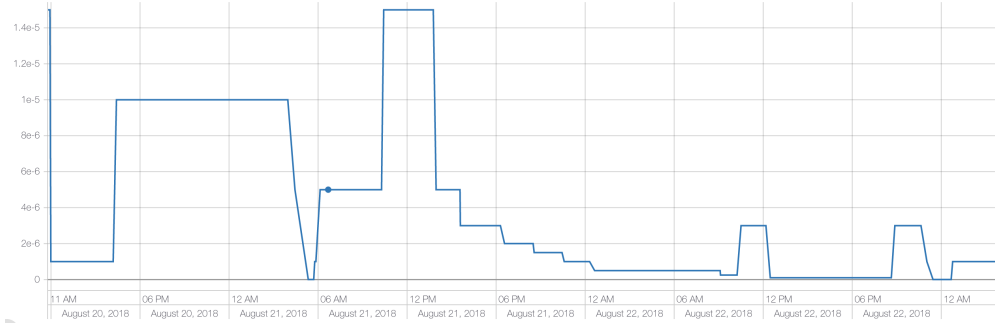
Figure 32: Learning Rate during The International: This is what happens when humans under time pressure choose hyperparameters. We believe that in the future automated systems should optimize these hyperparameters instead. After this event, our team began to internally refer to the act of frantically searching over hyperparameters as “designing skyscrapers.”
