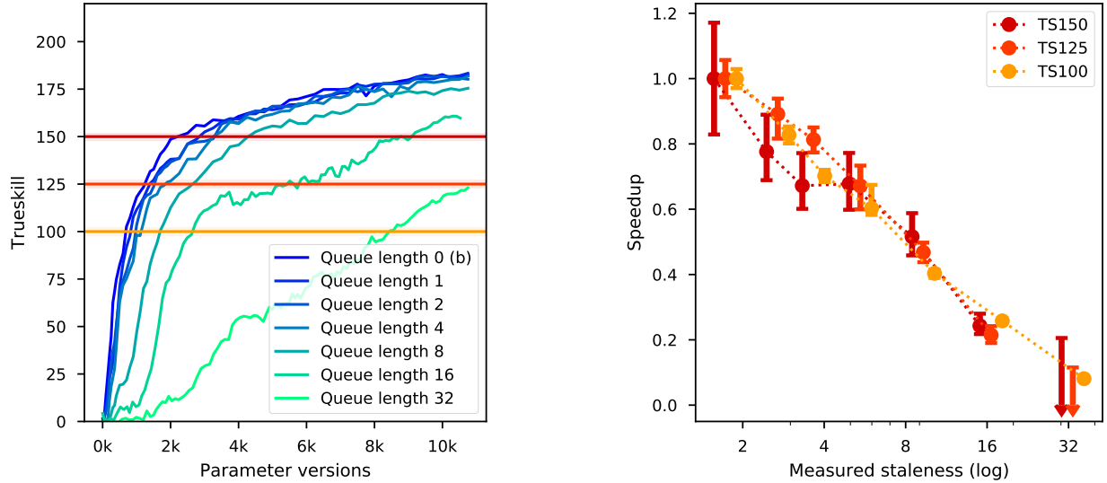
Figure 22: Effect of Staleness on training speed. (Replicated from main text Figure 5b) TrueSkill over the course of training (see Appendix J) and speedup measured by the rate to attain different TrueSkill thresholds (computed using Equation 2) granted by increasing Staleness. Increasing staleness of data causes significant losses in training speed.
