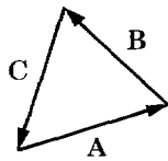
Figure 10.1.11 \mathbf{A} + \mathbf{B} + \mathbf{C} = \mathbf{0}
