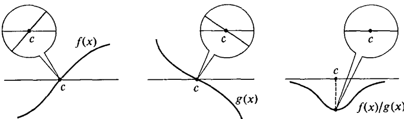
Figure 5.2.2 L'Hospital's Rule
