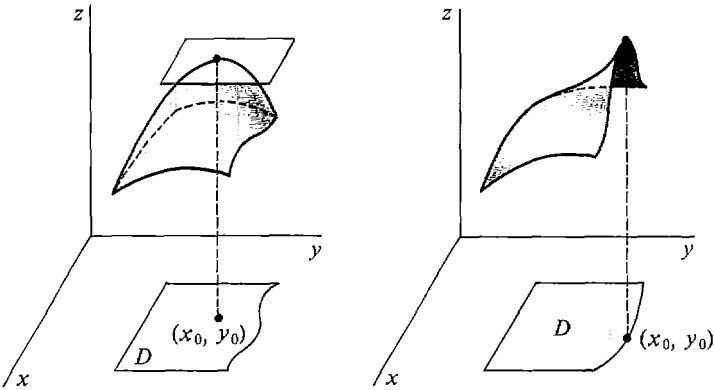
Case (i) Interior Maximum Case (ii) Boundary Maximum Figure 11.7.2 Critical Point Theorem
