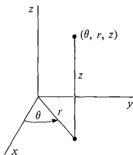
Cylindrical coordinates
