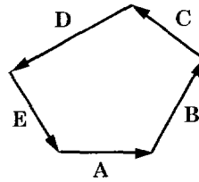
\mathbf{A} + \mathbf{B} + \mathbf{C} + \mathbf{D} + \mathbf{E} = \mathbf{0}
