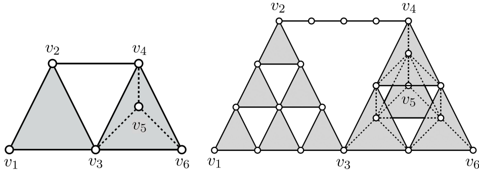
Fig. 2. \mathcal{H} and \mathcal{H}^{\frac{1}{f}}
