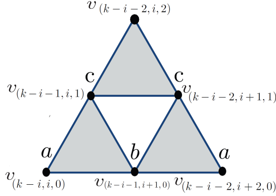
Fig. 3. \mathcal{H} and \mathcal{H}^{\frac{1}{T}}
