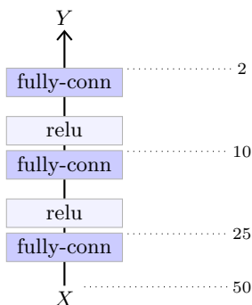
Figure 5.1: This multi-layer perceptron takes as input a one dimension tensor of size 50, is composed of three fully connected layers with outputs of dimensions respectively 25, 10, and 2, the two first followed by ReLU layers.
