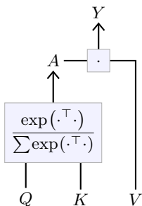
Figure 4.10: The attention operator Y = \text{att}(Q, K, V) computes first an attention matrix A as the per-query softmax of Q^\top K , and then computes the product between A and V . See Equation 4.3. This operator can be made causal by forcing all the upper-diagonal terms of the matrix A to zero before the normalization.
